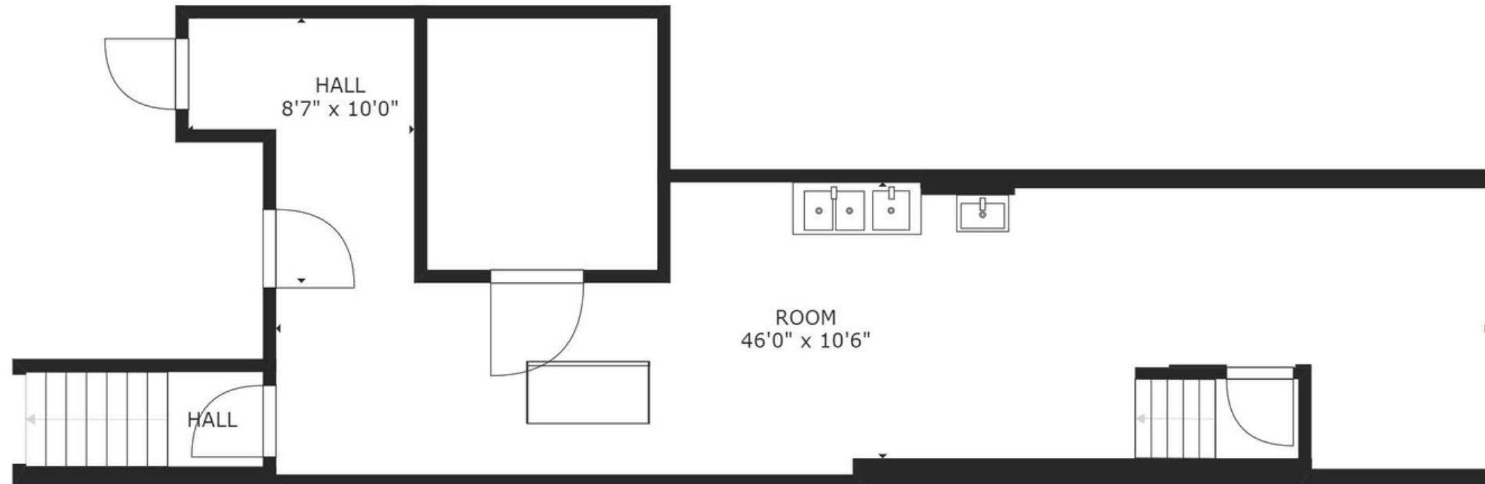
FLOOR 1
