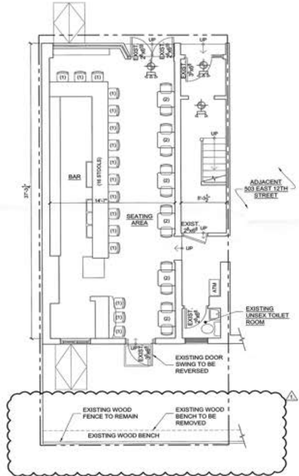
2 EXISTING/DEMO FIRST FLOOR PLAN SCALE: 1/4" = 1'-0"
